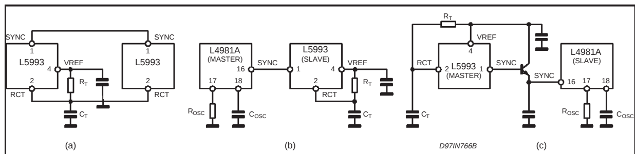
Figure 20. Synchronizing the L5993.
