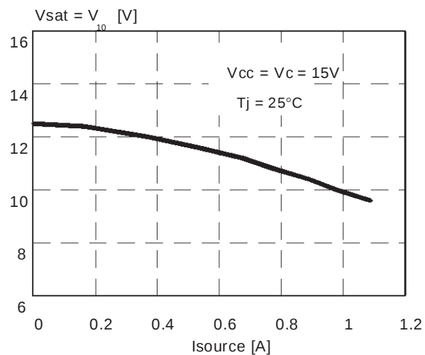
Figure 12. UVLO Saturation
